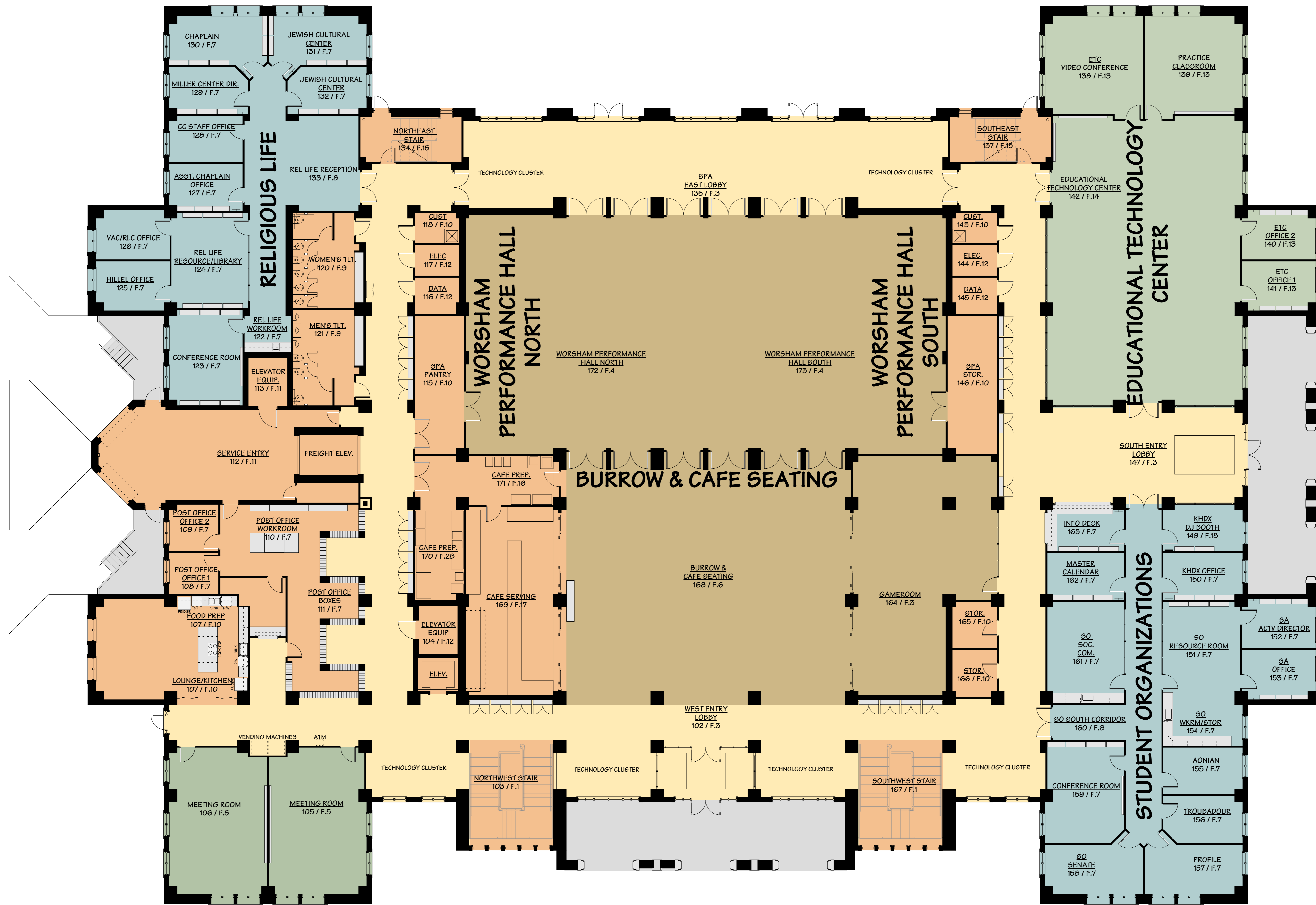
Hendrix College Student Life & Technology Center First Floor Plan - Kirchner Architecture, P.A.
